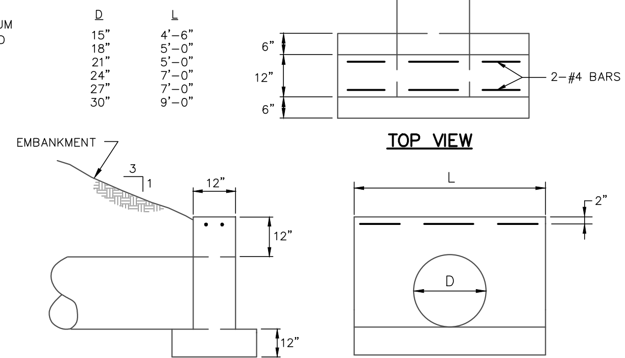
TYPICAL TYPE D ENDWALL NOT TO SCALE
