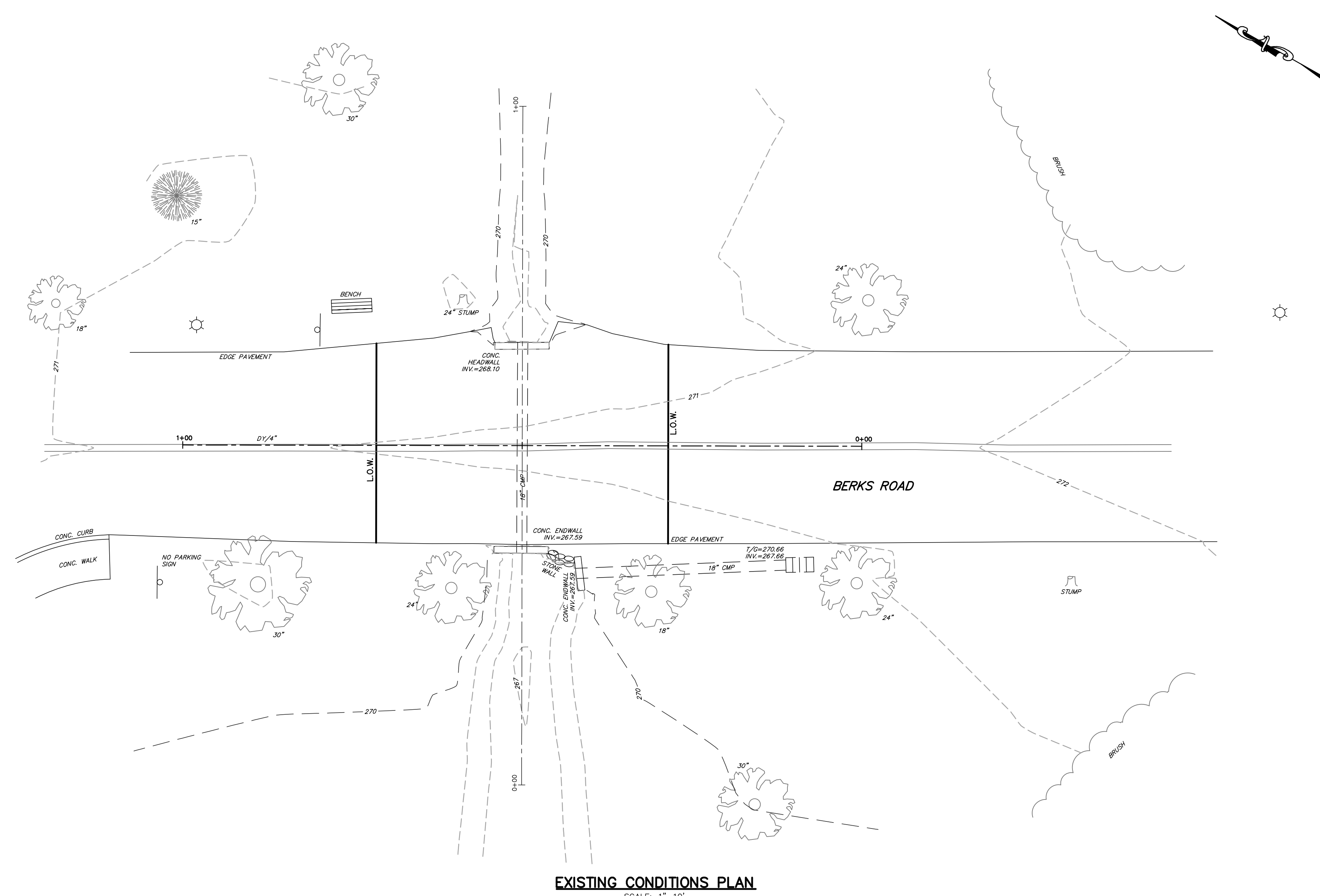
EXISTING CONDITIONS PLAN SCALE: 1"=10'
