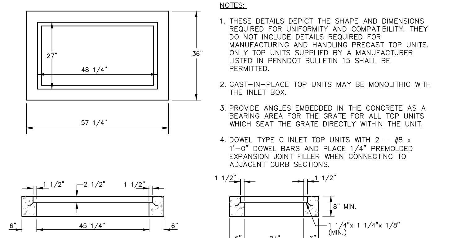
2'x4' TYPE M INLET CONCRETE TOP UNITS SCALE: NONE
