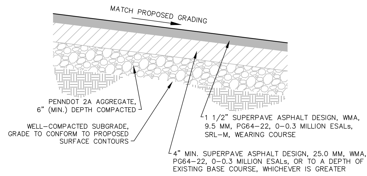
ACCESS DRIVE CROSS SECTION SCALE: NONE
