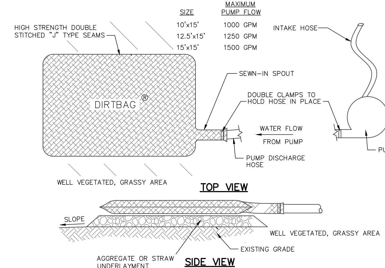
DIRTBAG FILTER BAG SCALE: NONE
