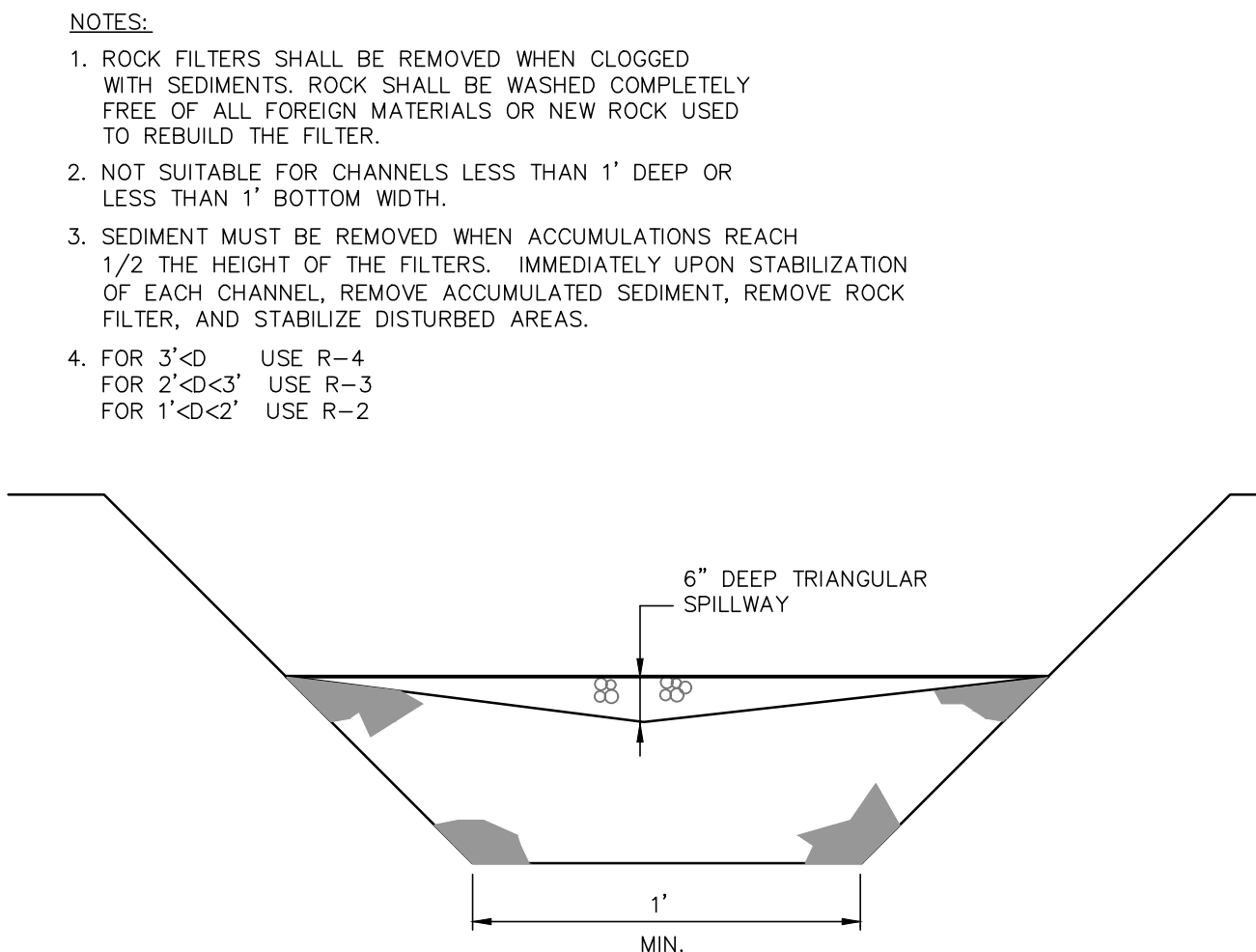
SECTION B-B
