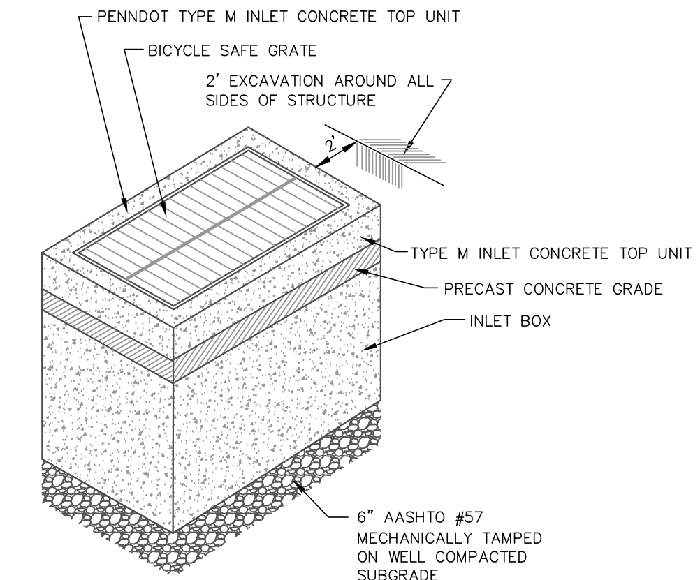
PRE-CAST STORM INLET-TYPE M SCALE: NONE
