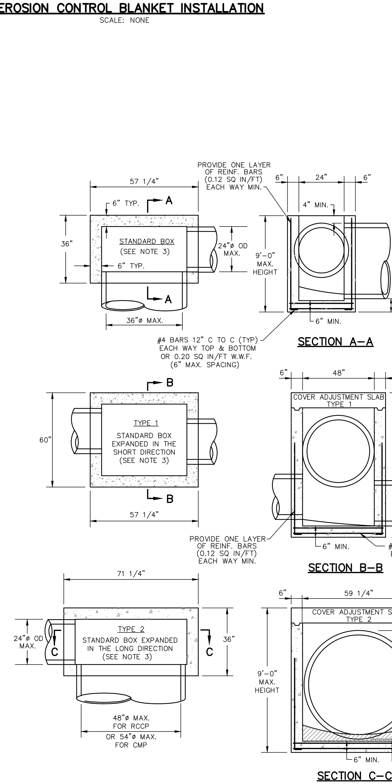
STANDARD PRECAST CONCRETE INLET BOXES SCALE: NONE
