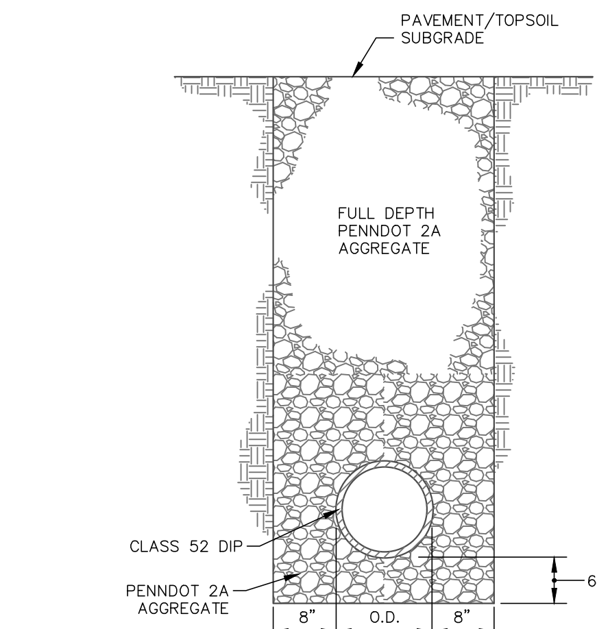
BEDDING AND BACKFILL DETAIL SCALE: NONE
