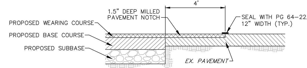
MILLED PAVEMENT NOTCH SCALE: NONE
